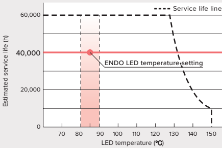
Relationship graph between LED temperature and service life
