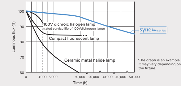
Comparison data of luminous flux maintenance rate
