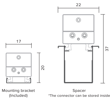
Fixture size (mm)
