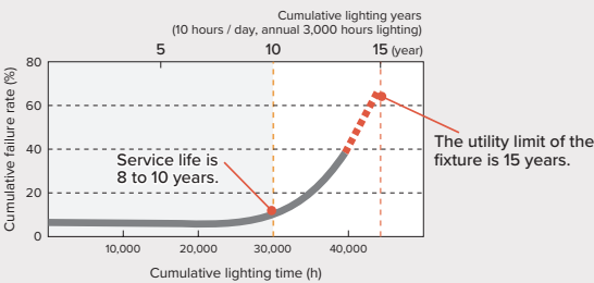
Cumulative failure rate of lighting fixtures
