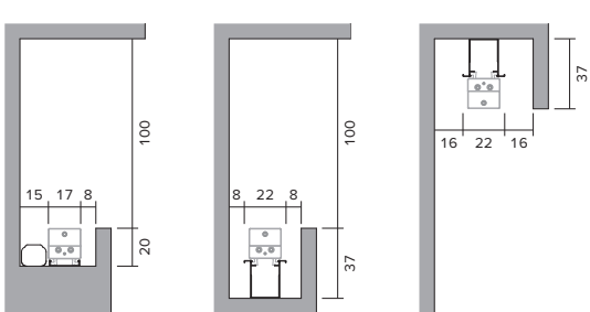
Minimum required installation (mm)
